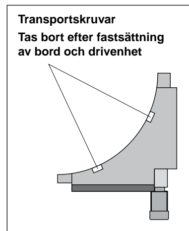
Figur 2 Transportskruvar
